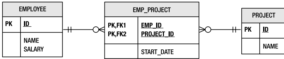
Figure 8-10. Join table with additional state
